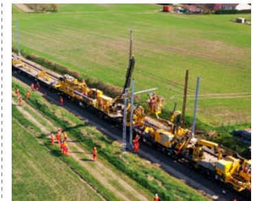
TSO high-capacity train in the 25-kilovolt network
